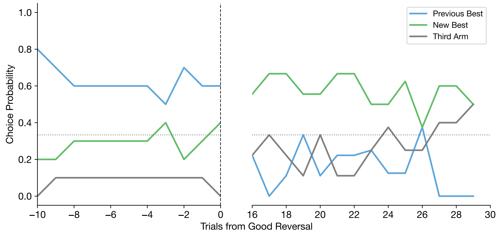
Good Reversal-Aligned Choices (mean \pm se across subjects | n=1 subjects, n=10 reversals) (Skipping first 15 trials post-reversal)
